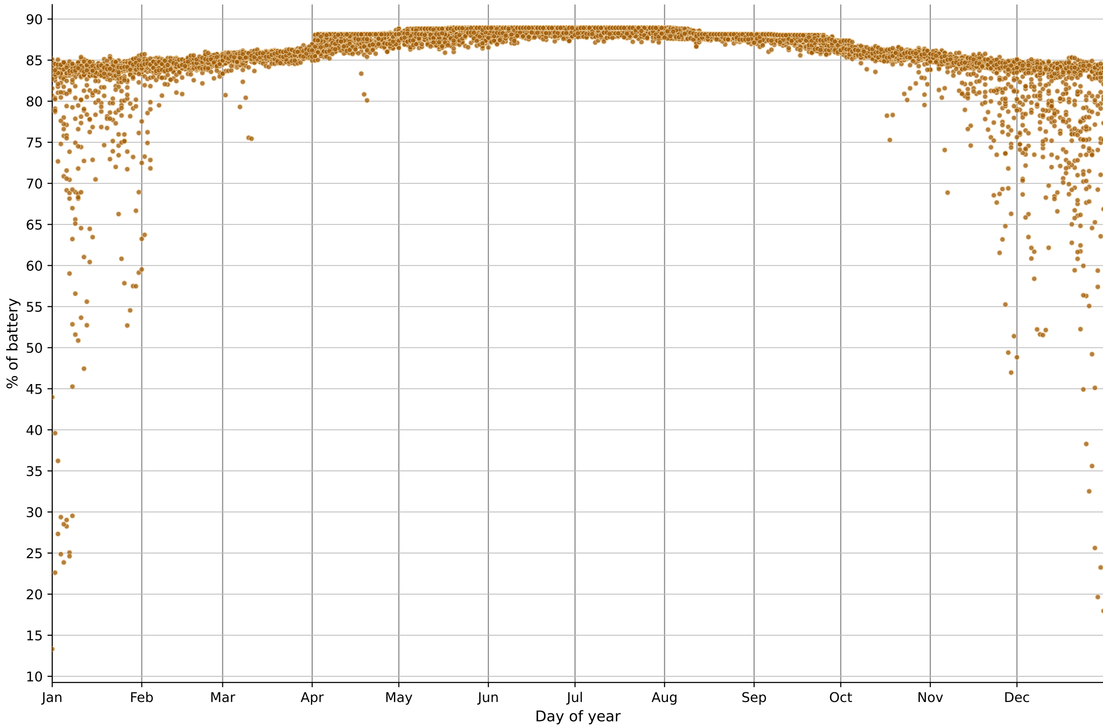
Battery min charge state per day (176.8 kWh = 100 %) Austria - Inning 48.18200, 15.41700
