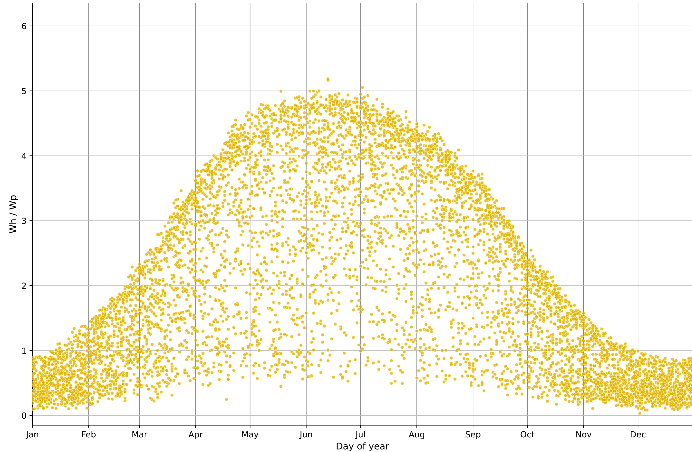
Yield distribution for each day — W_h / W_p of all PV together Austria - Inning 48.18200, 15.41700
