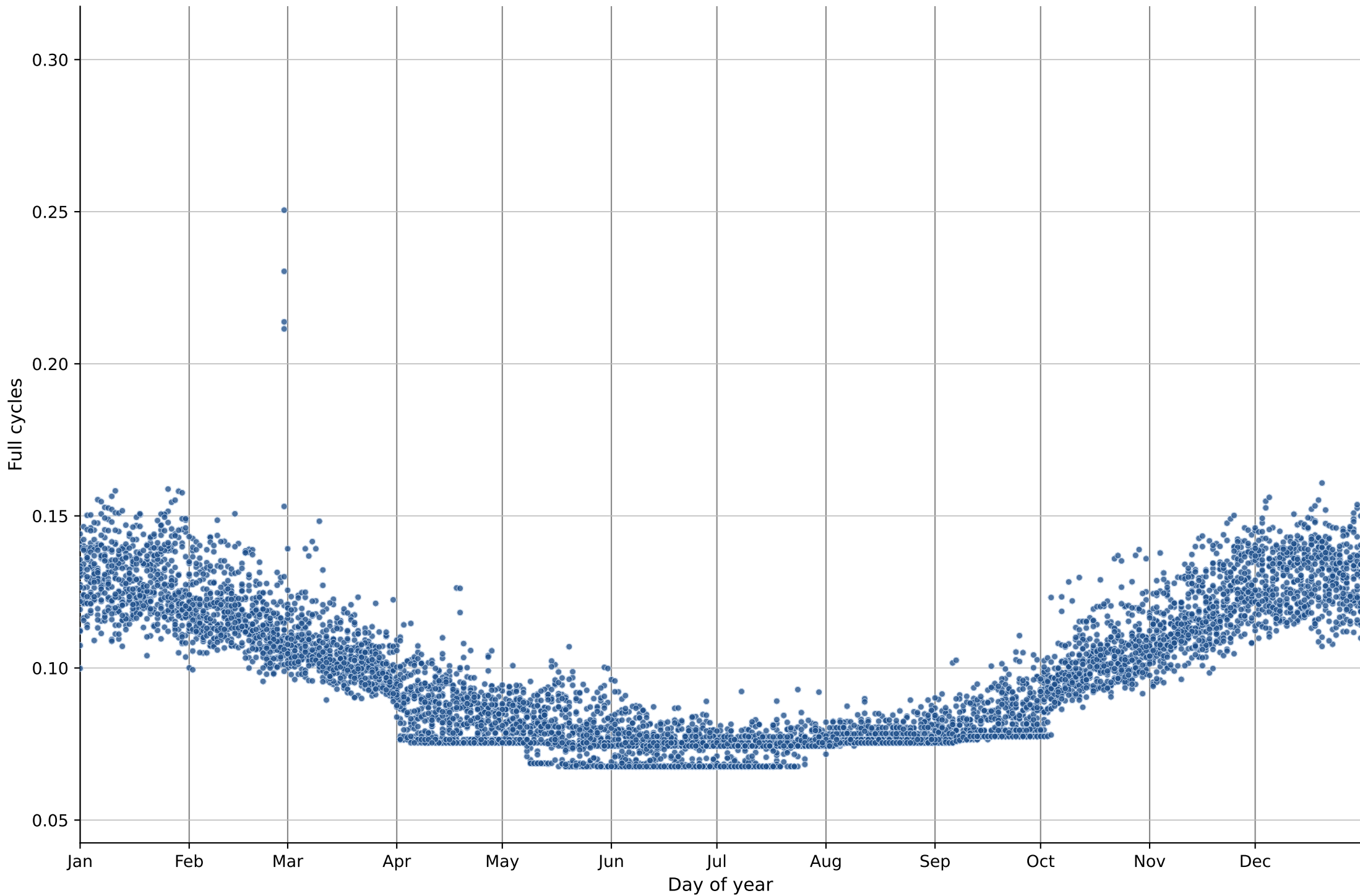
Battery cycles per day (discharge / 176.8 kWh) Austria - Inning 48.18200, 15.41700
