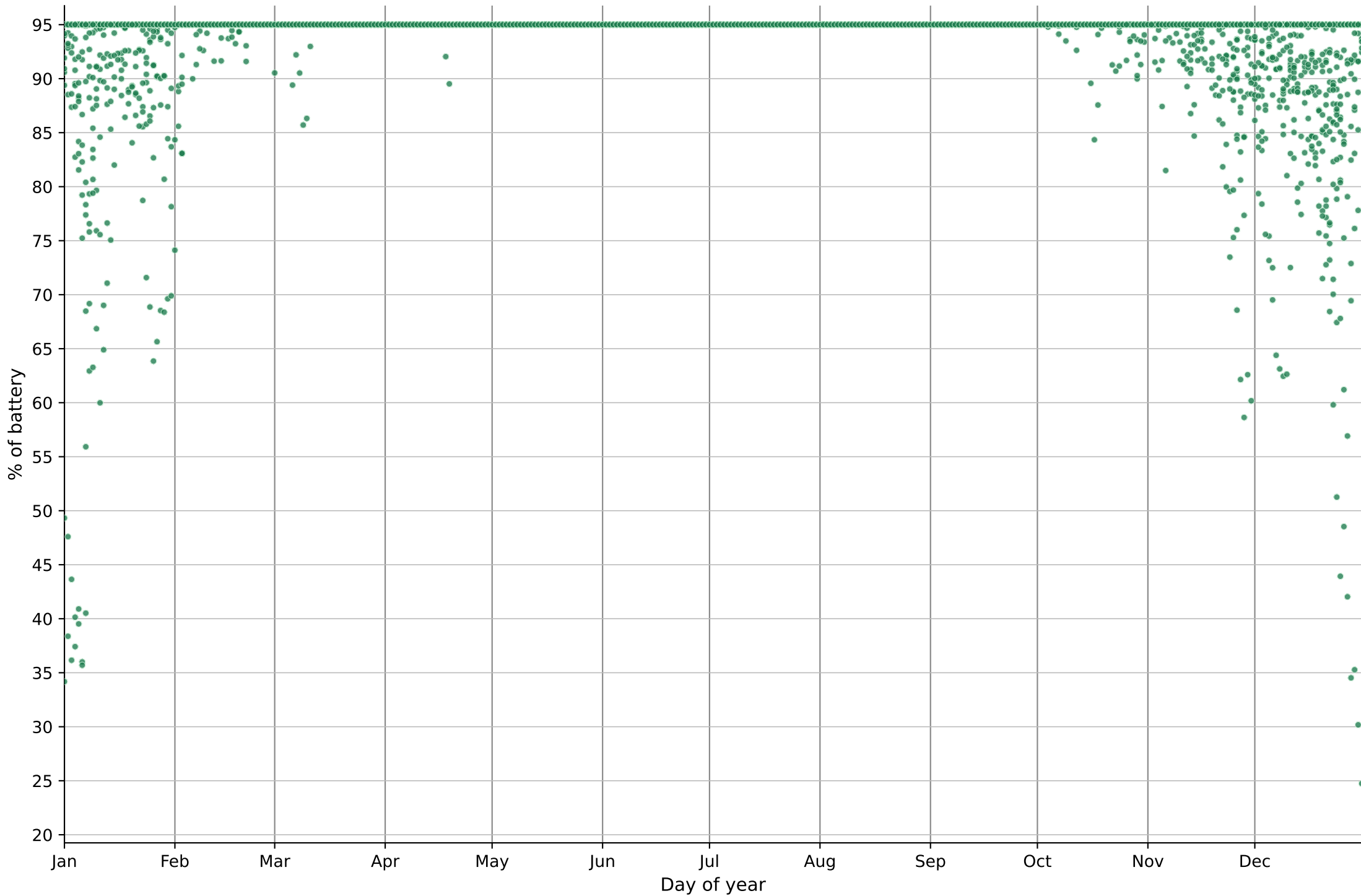
Battery max charge state per day (176.8 kWh = 100 %) Austria - Inning 48.18200, 15.41700
