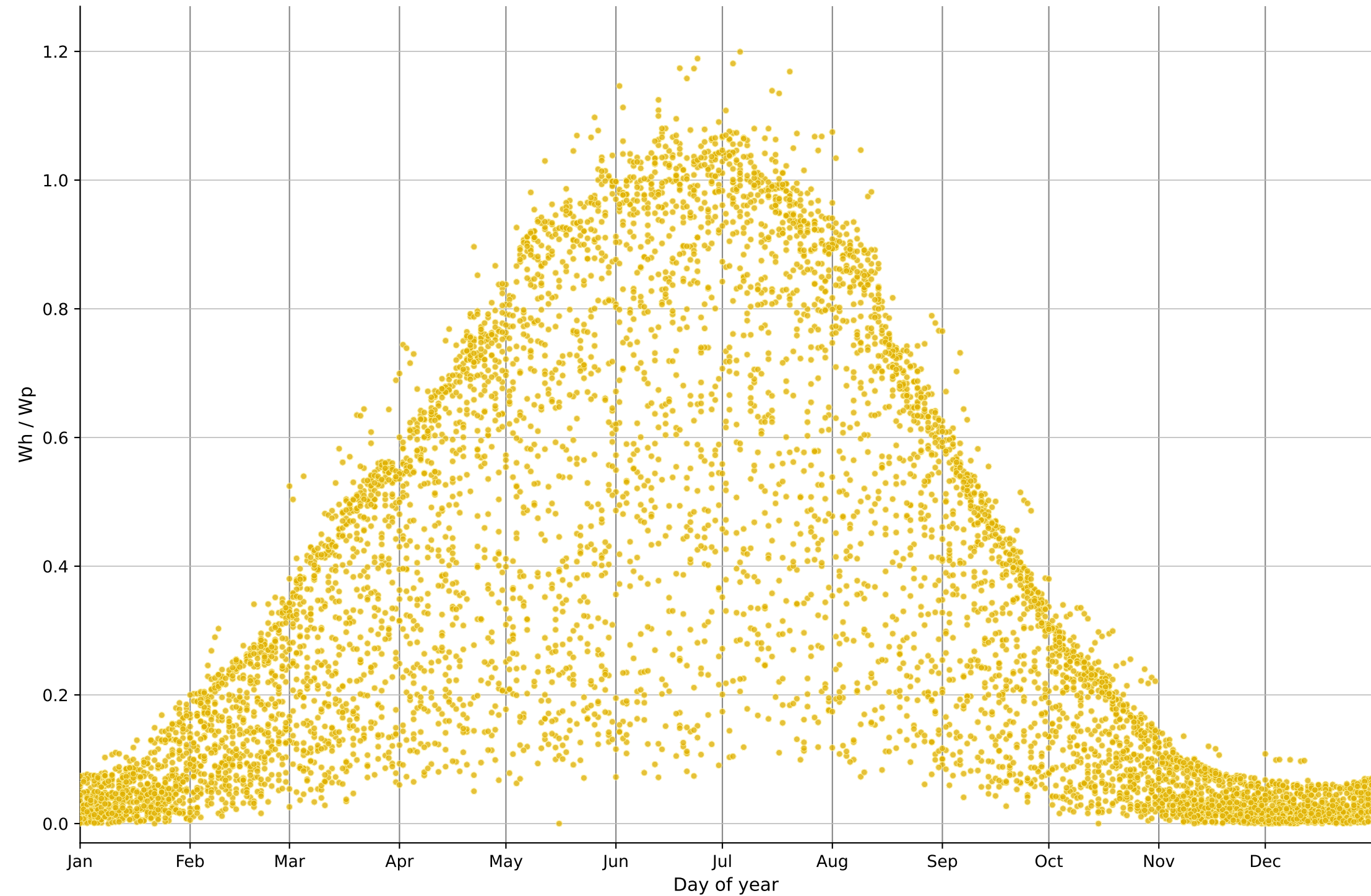
Yield distribution for each day — Wh / Wp of all PV together — 15:00-23:59 Austria - Inning 48.18200, 15.41700
