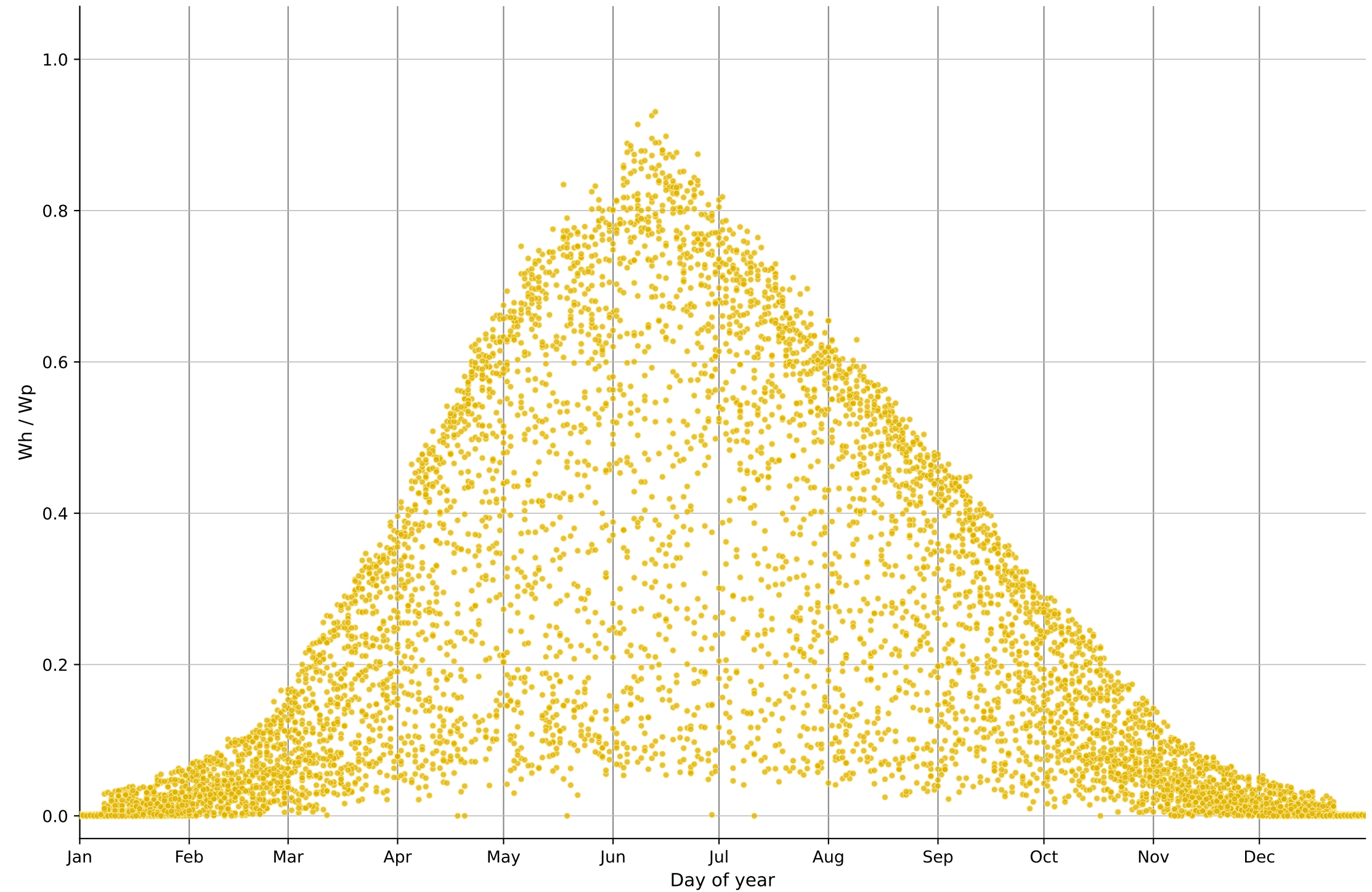
Yield distribution for each day — Wh / Wp of all PV together — 00:00-09:00 Austria - Inning 48.18200, 15.41700
