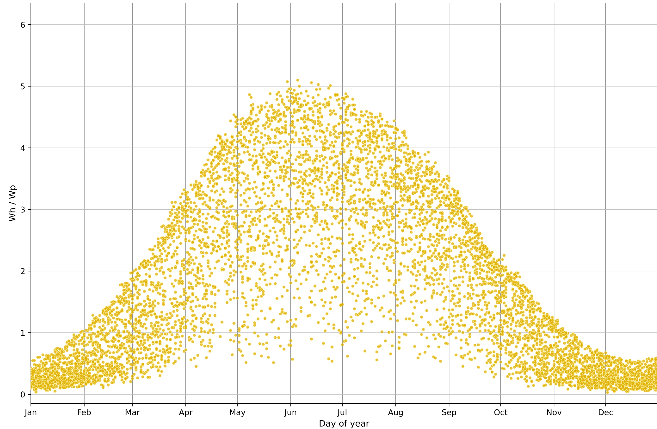
Yield distribution for each day — W_h / W_p of all PV together Germany - Grünheide 52.40100, 13.84200
