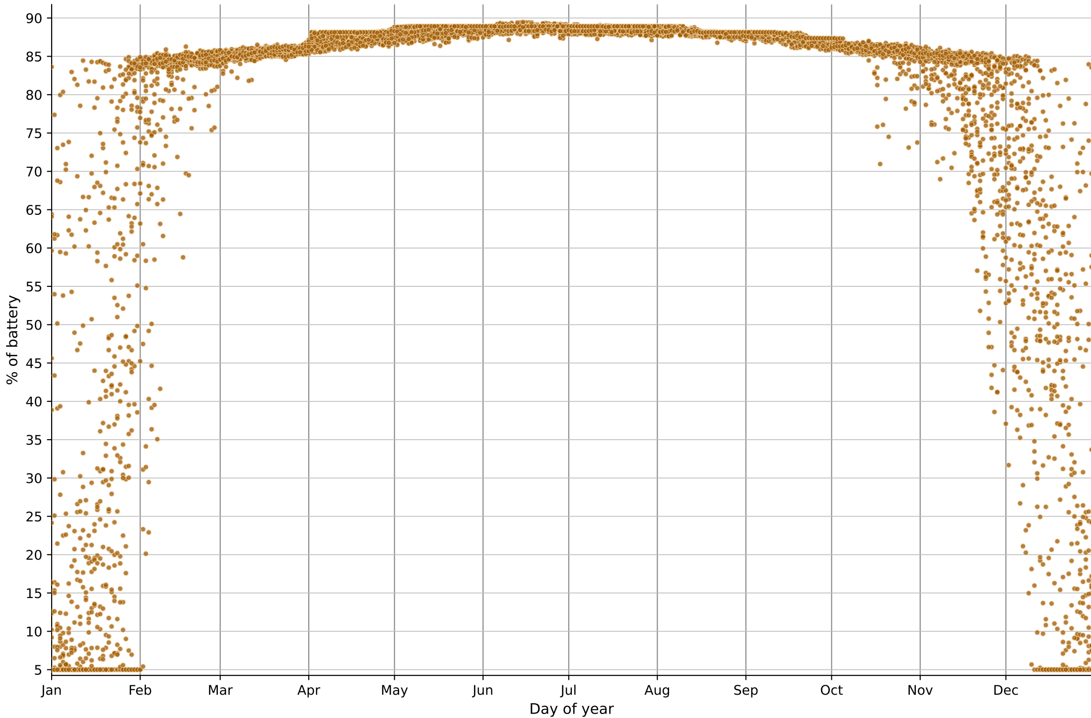
Battery min charge state per day (176.8 kWh = 100 %) Germany - Grünheide 52.40100, 13.84200
