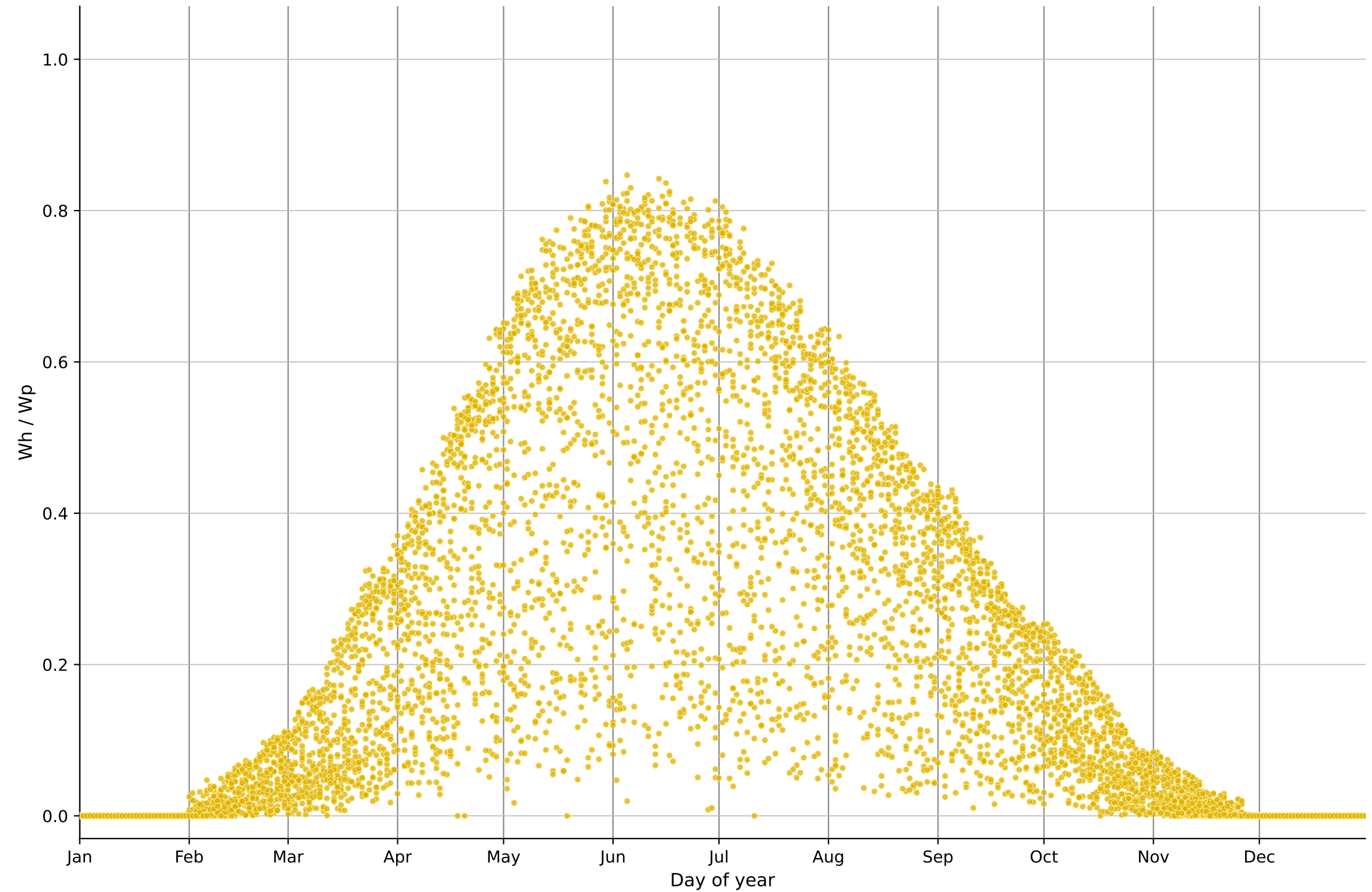
Yield distribution for each day — Wh / Wp of all PV together — 00:00-09:00 Germany - Grünheide 52.40100, 13.84200
