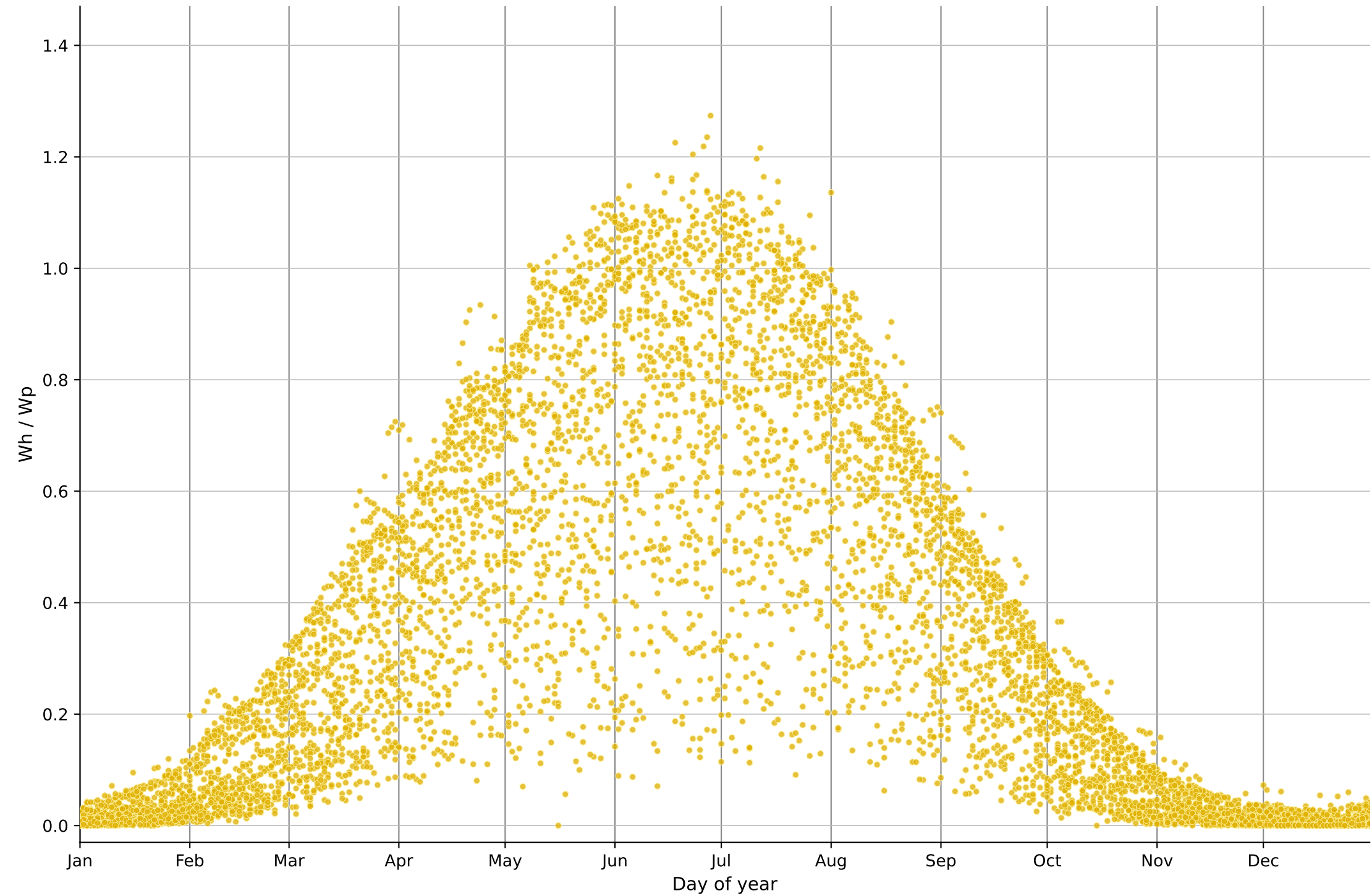
Yield distribution for each day — Wh / Wp of all PV together — 15:00-23:59 Germany - Grünheide 52.40100, 13.84200
