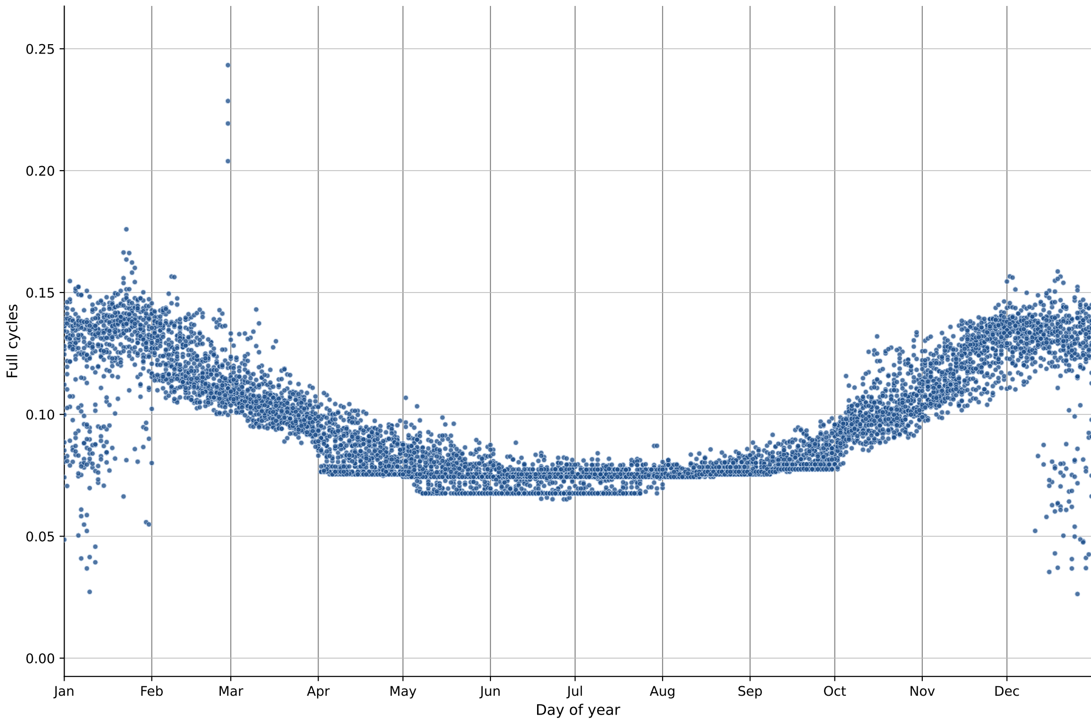
Battery cycles per day (discharge / 176.8 kWh) Germany - Grünheide 52.40100, 13.84200
